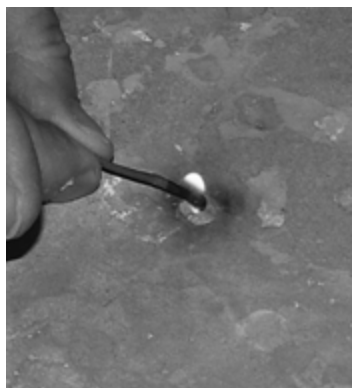
Flame is pulled into the kiln
