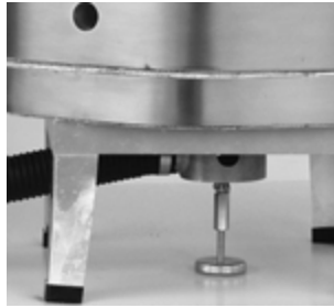
Under kiln mount with height adjustment
