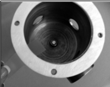
Gasket installed on collector cup (use tape to keep in place)
